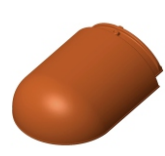
Ridge Beginner No. 3001 Cover length: approx. 385 mm Cover width: approx. 275 mm Weight: approx. 5,2 kg
